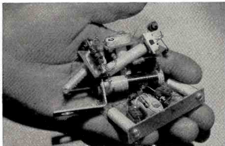
Just a handful of parts need be installed for color conversion of internal circuits. A G-E transmitter incorporating these changes will be exhibited at NARTB. See this convention feature in operation. Make the General Electric booth your first stop.
