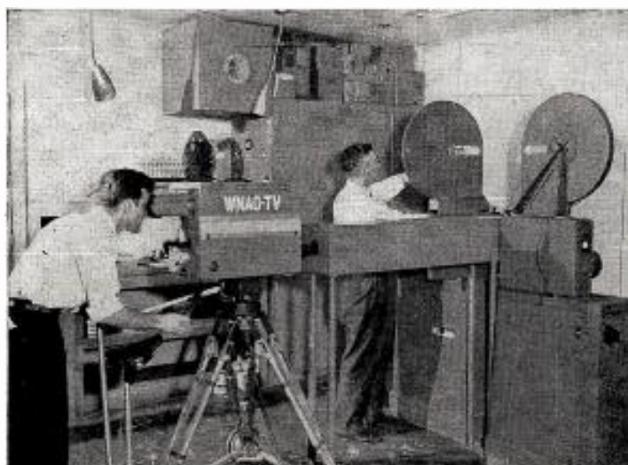
Engineers W. F. Anderson and L. E. Rudisill set up the late evening film show on WNAO's General Precision Laboratories 16mm projectors. The FTL image orthicon camera is also used for interviews and newscasts originating "live" in a small studio here at the transmitter building.
